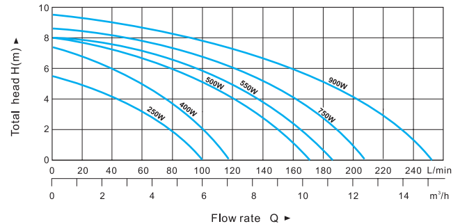
PERFORMANCE CHART AT n=2900 r/min
