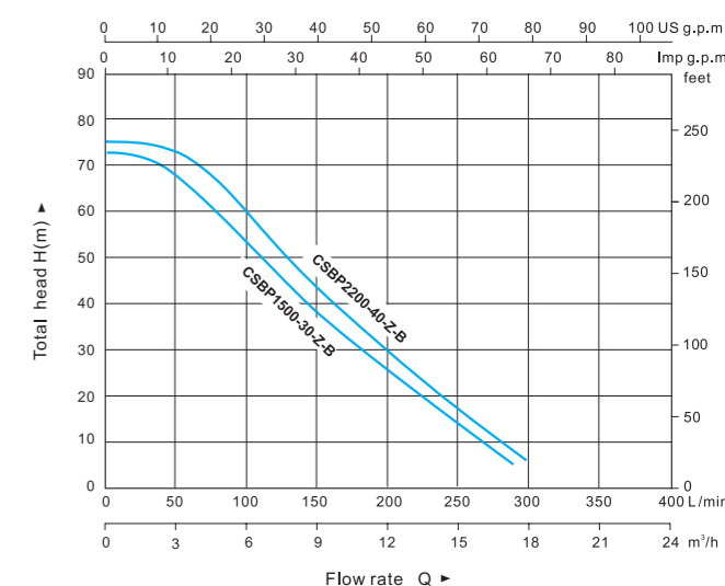
PERFORMANCE CHART AT n=2900 r/min
